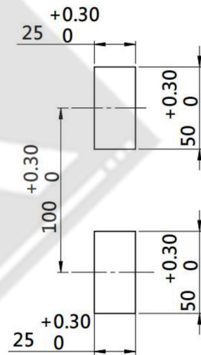
PANEL CUTOUT
